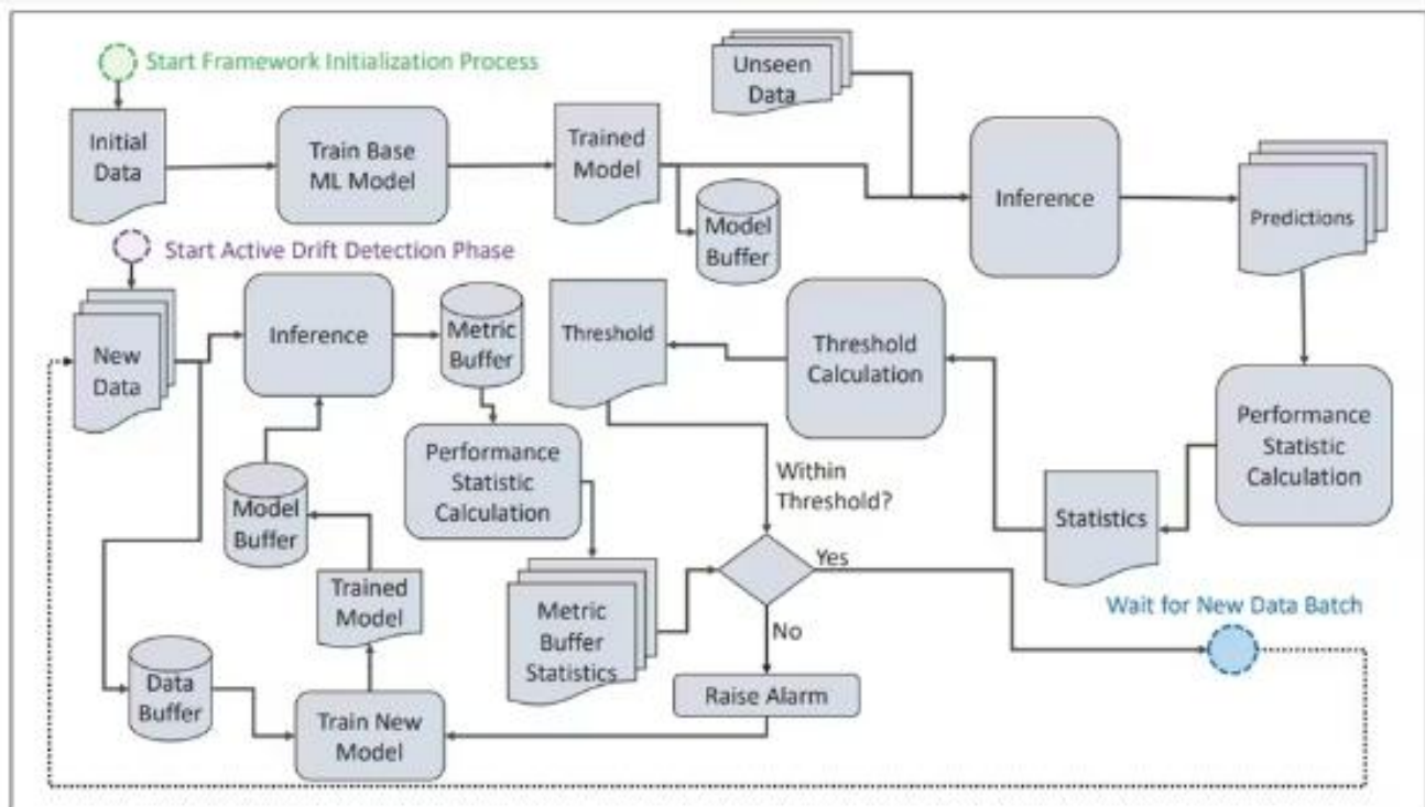
Figure 2 Drift detection and adaptation framework
