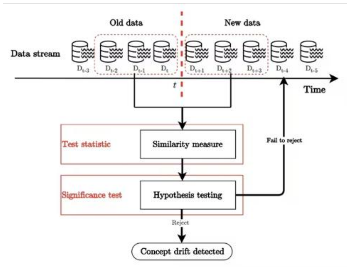
Figure 1 Concept Drift Detection Framework
